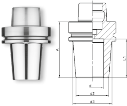
HSK63F-Schrumpffutter HSK63F-Induction shrink chuck
